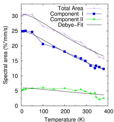
Figure 2.3: The spectral area of the components I and II in the first step of the fitting procedure and the corresponding Debye fits used for the second step.
