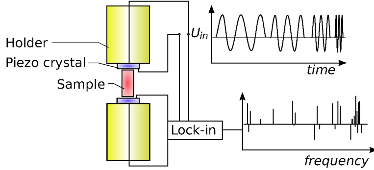
Figure 1.17: Schematic representation of RUS setup. The generated sinus shape signal is applied as pressure waves to the sample via the piezoelectric crystal. The resulting deformation is converted into an electric signal via the second piezoelectric crystal and a Lock-in amplifier. The obtained results are the resonances frequencies of the sample.
